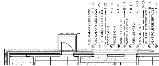
3 TYPICAL SITE LIGHTING CIRCUITS 3/16" = 1'-0"
