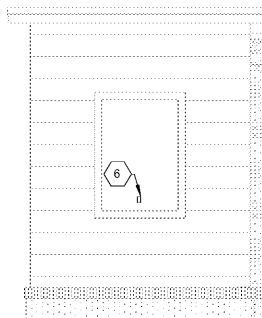
2 CORNER TOWER FRONT ELEVATION 3/16" = 1'-0"
