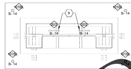
4 FRONT ENTRY TOWER LIGHTING 3/16" = 1'-0"
