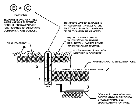
2 DETAIL - CONCRETE MARKER DETAIL SCALE: NONE
