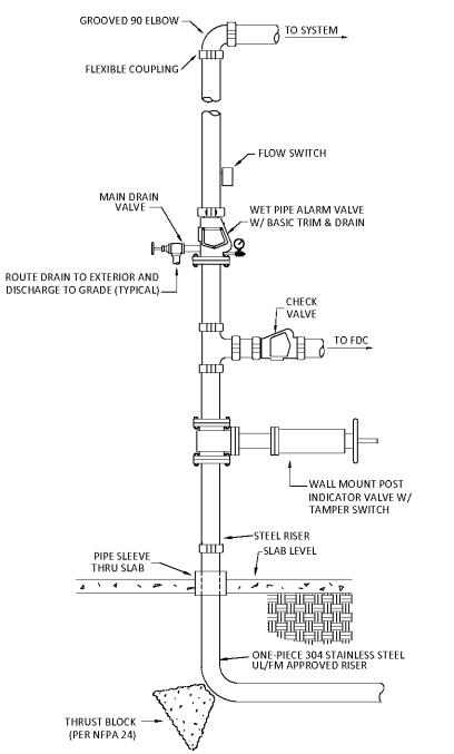
3 FIRE SPRINKLER RISER NOT TO SCALE
