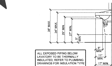
14 LAVATORY CLEARANCES A4.1 SCALE: 1/2" = 1'-0"
