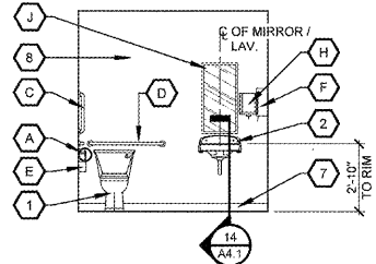
7 WOMEN'S ELEVATION A4.1 SCALE: 1/4" = 1'-0"
