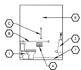
2 MEN'S ELEVATION A4.1 SCALE: 1/4" = 1'-0"
