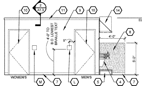
10 RESTROOM ELEVATION A4.1 SCALE: 1/4" = 1'-0"
