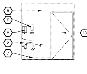
8 WOMEN'S ELEVATION A4.1 SCALE: 1/4" = 1'-0"
