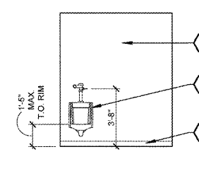
5 MEN'S ELEVATION A4.1 SCALE: 1/4" = 1'-0"
