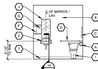
3 MEN'S ELEVATION A4.1 SCALE: 1/4" = 1'-0"
