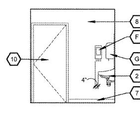
4 MEN'S ELEVATION A4.1 SCALE: 1/4" = 1'-0"
