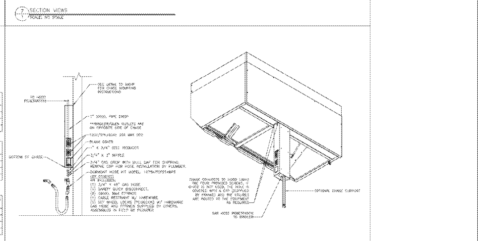
TYPICAL GAS AND ELECTRICAL CHASE DETAILS SCALE: AS SHOWN
