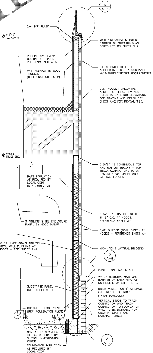
4 KITCHEN HOOD WALL
