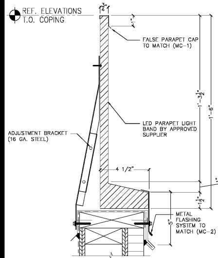
A PARAPET LIGHT BAND DETAIL
