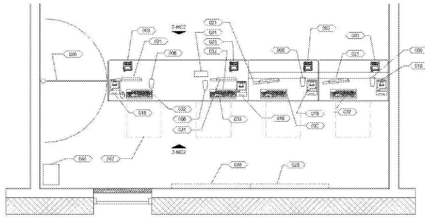
1 (LEFT) EQUIPMENT PLAN 1/4" = 1'-0"
