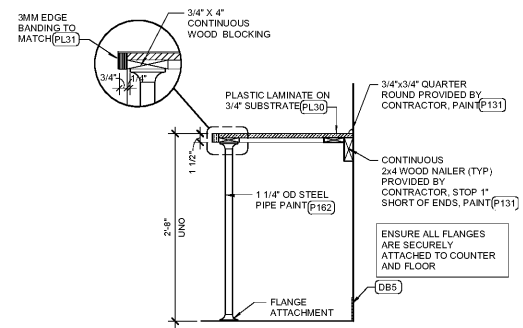
8 COUNTER SECTION 1" = 1'-0"
