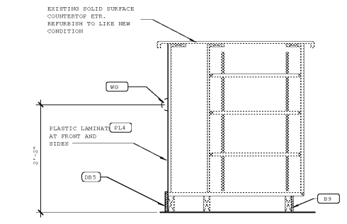
4 BASE CABINET SECTION (AT ACC) 1" = 1'-0"
