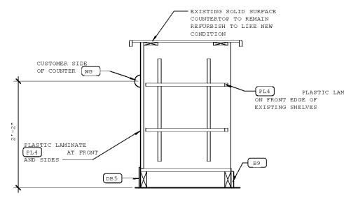
3 BASE CABINET SECTION 1" = 1'-0"
