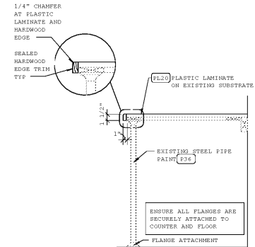
2 COUNTER SECTION 1" = 1'-0"
