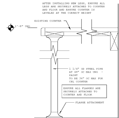
1 COUNTER LEG 3" = 1'-0"
