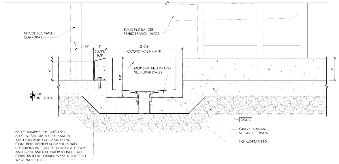
B1 Interior Section Detail - EVAC Floor Sink (Front) SCALE: 1 1/2" = 1'-0"
