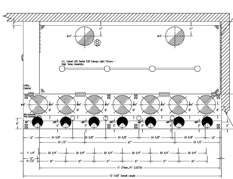
PLAN VIEW - Hood #1 11' 2.00" LONG 5430ND-2-ACPSP-F
