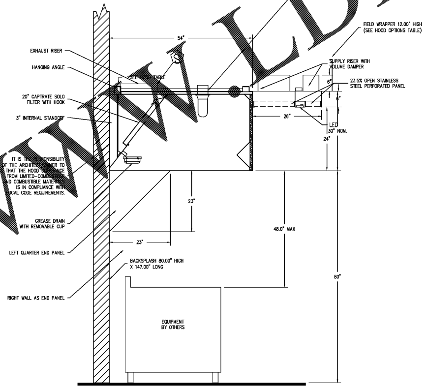
SECTION VIEW - MODEL 5430ND-2-ACPSP-F HOOD - #1
