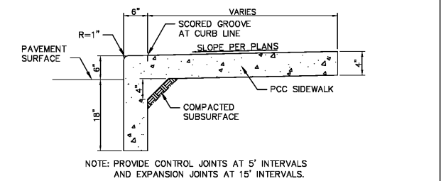
TURN DOWN CURB AND SIDEWALK NOT TO SCALE
