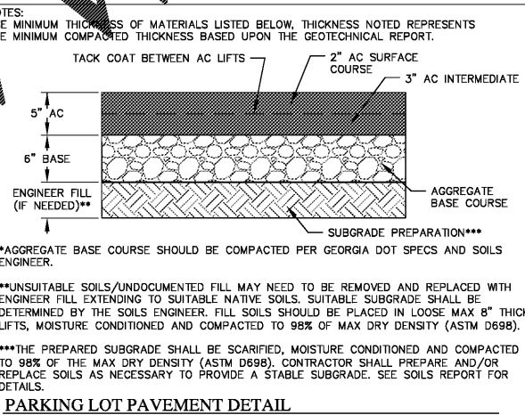
PARKING LOT PAVEMENT DETAIL NOT TO SCALE
