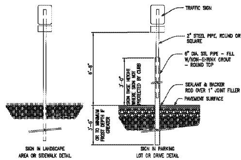
SIGN POST DETAIL NOT TO SCALE
