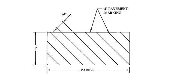
PEDESTRIAN ACCESS PAVEMENT MARKING DETAIL NOT TO SCALE
