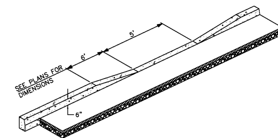
CURB TAPER DETAIL NOT TO SCALE
