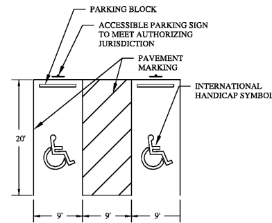
ACCESSIBLE PARKING SPACE DETAIL NOT TO SCALE
