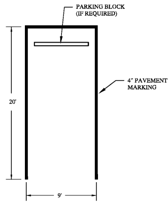
PARKING SPACE DETAIL NOT TO SCALE
