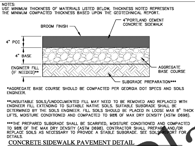
CONCRETE SIDEWALK PAVEMENT DETAIL NOT TO SCALE
