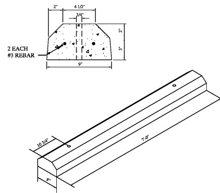
PARKING BLOCK DETAIL NOT TO SCALE
