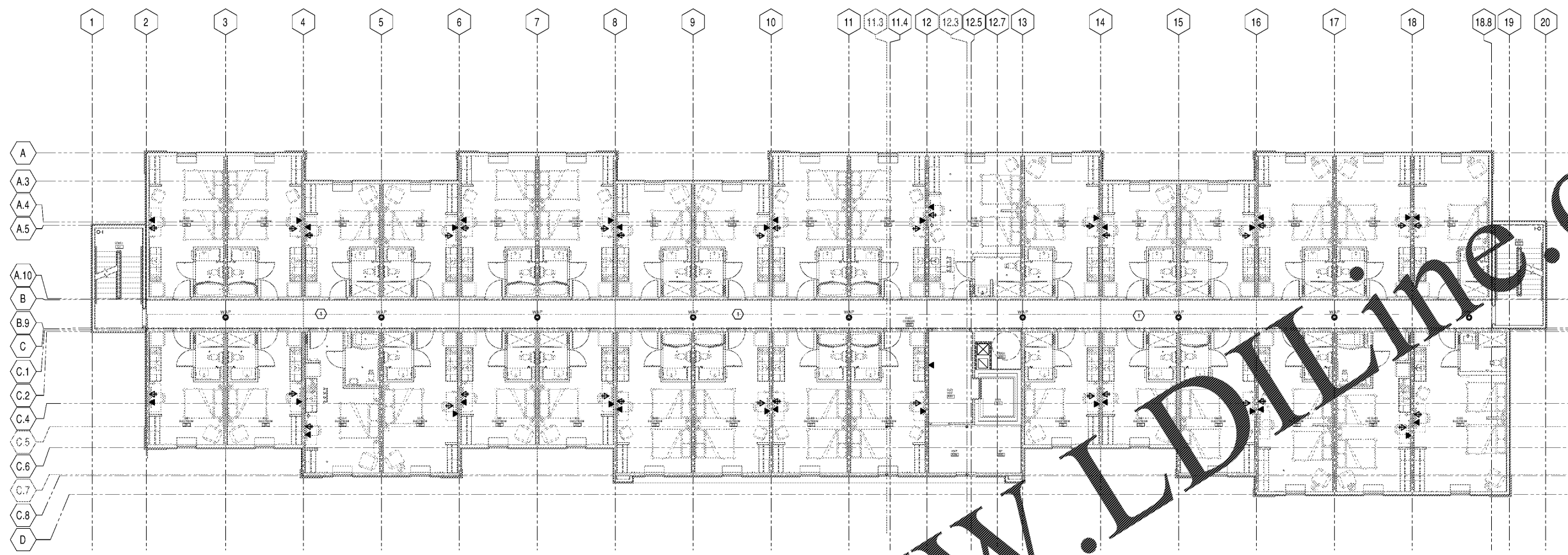
1 LEVEL THREE FLOOR PLAN - LOW VOLTAGE SYSTEMS 1/8" = 1'-0"
