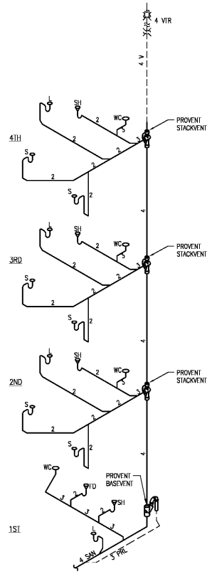
2 WASTE & VENT DIAGRAM NO SCALE
