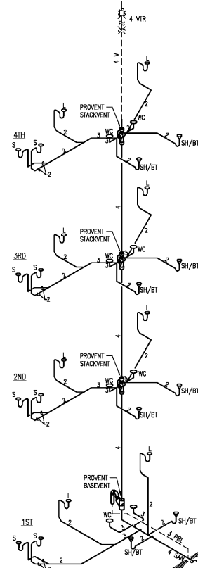
3 WASTE & VENT DIAGRAM NO SCALE
