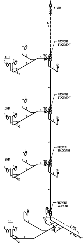
1 WASTE & VENT DIAGRAM NO SCALE
