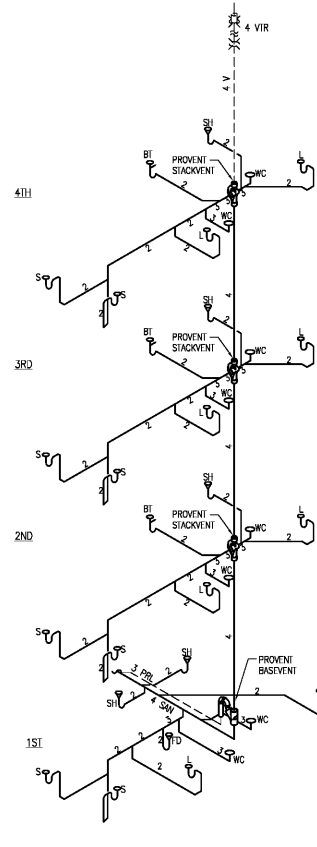
9 WASTE & VENT DIAGRAM NO SCALE
