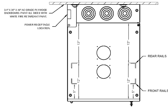
WALL MOUNT PLAN VIEW LEFT HINGE
