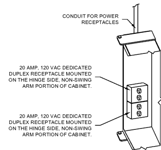
TR CABINET POWER BACK PANEL HINGED SIDE VIEW
