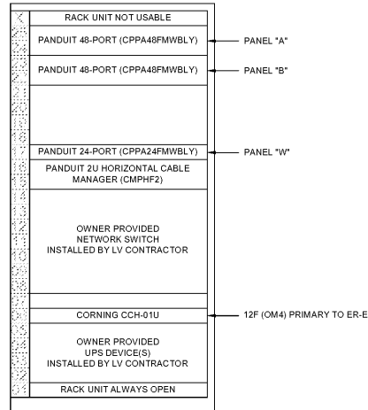
WALL MOUNT ELEVATION VIEW - FRONT RAILS
