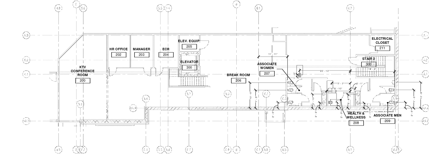
1 PLUMBING MEZZANINE DIMENSION PLAN 1/8" = 1'-0"
