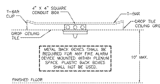
CEILING HORN/STROBE FLUSH MOUNTING DETAIL SCALE: NO SCALE
