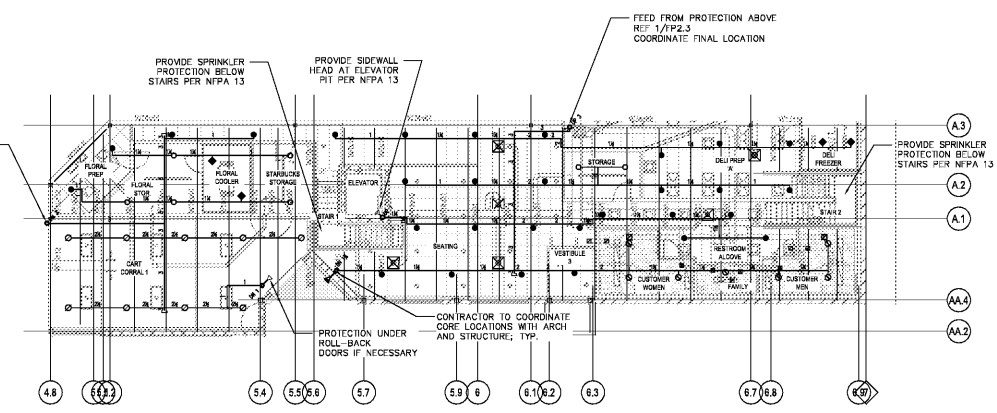
2 LOWER LEVEL SPRINKLER PLAN SYSTEM 3 SCALE: 3/32" = 1"
