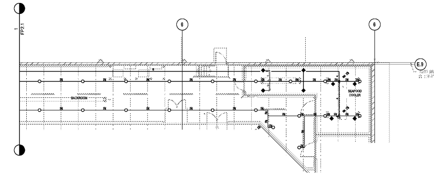
2 SPRINKLER PLAN SYSTEM 1 SCALE: 3/32" = 1'
