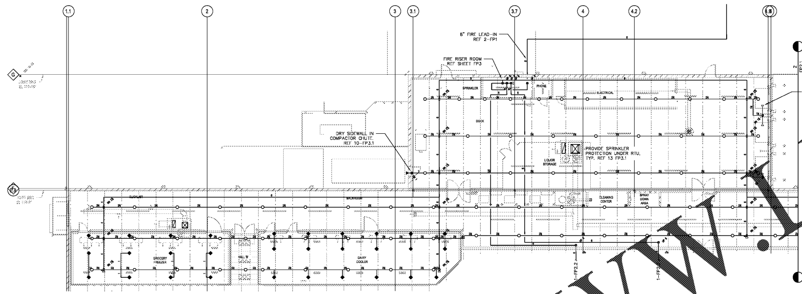
1 SPRINKLER PLAN SYSTEM 1 SCALE: 3/32" = 1'
