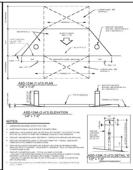
RAMP AT PEDESTRIAN CROSSING DATE: 8/8/11 DRAWN: ZAW ORIGINAL ISSUE DATE: 2/20/06 MASTER SPECIFICATION DETAIL ASD-124A
