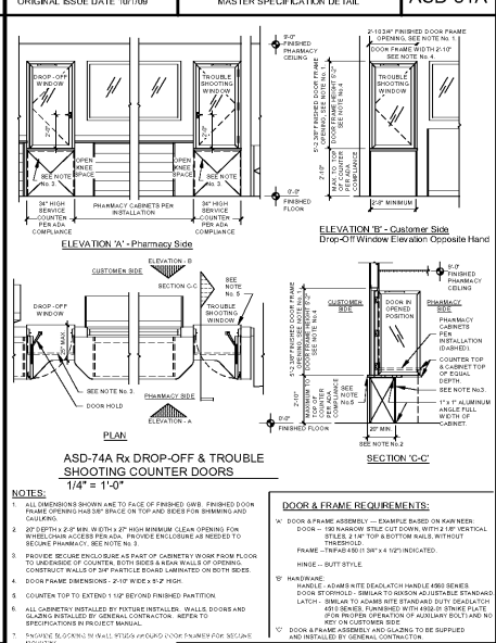
RxDROP-OFF & TROUBLE SHOOTING WINDOW COUNTER DOORS DATE: 7/11/16 DRAWN: ZAW ORIGINAL ISSUE DATE: 6/22/16 MASTER SPECIFICATION DETAIL ASD-74A
