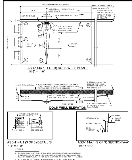
DELIVERY DOCK WITHOUT COMPACTOR AT RECESSED TRUCK WELL DATE: 11/29/15 DRAWN: ZAW ORIGINAL ISSUE DATE: 8/17/07 MASTER SPECIFICATION DETAIL ASD-114A
