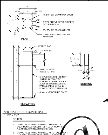
LIFT-OUT GUARD RAIL DATE: 11/7/11 DRAWN: ZAW ORIGINAL ISSUE DATE: 11/17/11 MASTER SPECIFICATION DETAIL ASD-91A
