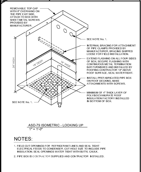
PREFABRICATED SHEET METAL BOX FOR MECHANICAL PIPING DATE: 5/13/13 DRAWN: ZAW ORIGINAL ISSUE DATE: 4/11/07 MASTER SPECIFICATION DETAIL ASD-79
