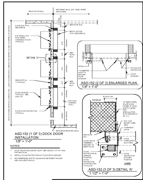
DOCK DOORS INSTALLATION DATE: 1/30/15 DRAWN: ZAW ORIGINAL ISSUE DATE: 2/20/06 MASTER SPECIFICATION DETAIL ASD-152
