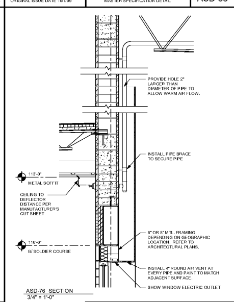
FRONT WALL FOR SPRINKLER ACCESS DATE: 11/7/16 DRAWN: ZAW ORIGINAL ISSUE DATE: 11/7/16 MASTER SPECIFICATION DETAIL ASD-76
