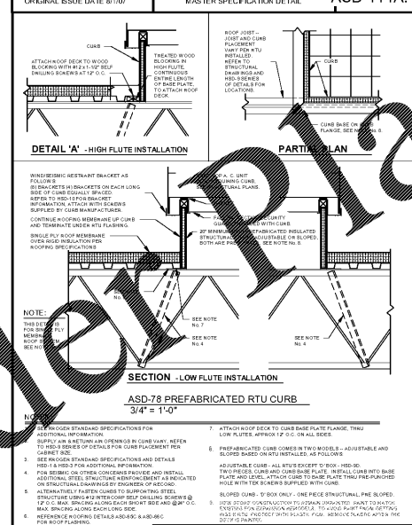
PREFABRICATED RTU CURB DATE: 11/7/16 DRAWN: ZAW ORIGINAL ISSUE DATE: 2/20/06 MASTER SPECIFICATION DETAIL ASD-78
