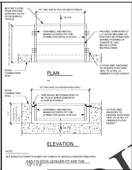
DOCK LEVELER PIT AND TUB DATE: 2/20/06 DRAWN: ZAW ORIGINAL ISSUE DATE: 2/20/06 MASTER SPECIFICATION DETAIL ASD-115
