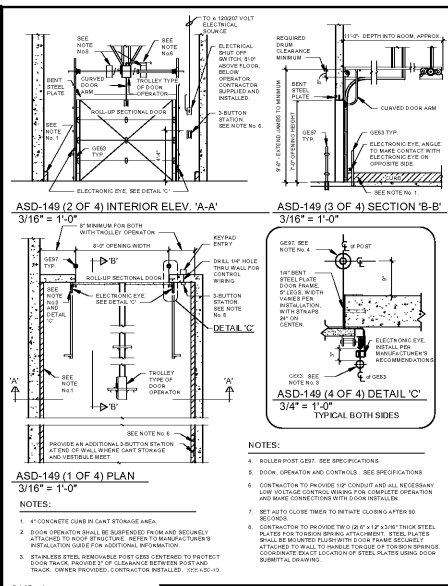
BASCART DOOR INSTALLATION WITH TROLLEY DOOR OPERATOR DATE: 8/8/11 DRAWN: ZAW ORIGINAL ISSUE DATE: 4/15/11 MASTER SPECIFICATION DETAIL ASD-149
