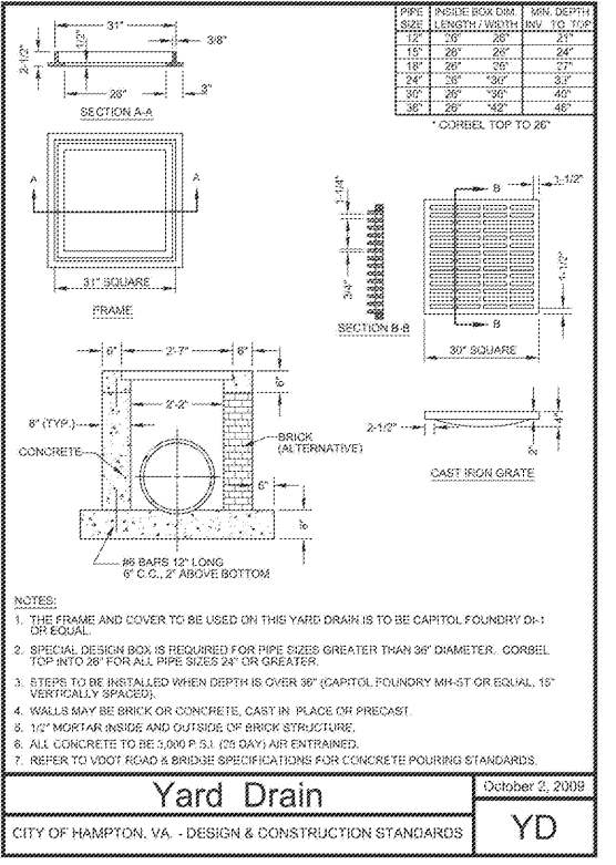
YARD DRAIN NOT TO SCALE C-620 1
