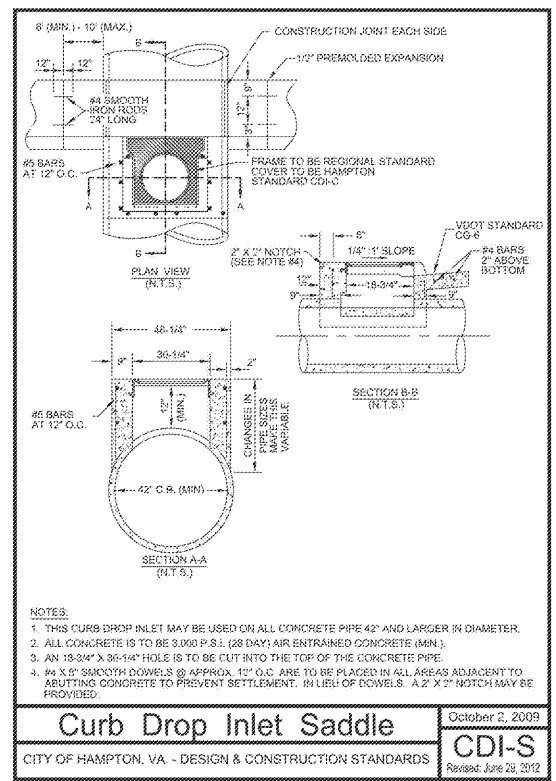
CURB DROP INLET SADDLE NOT TO SCALE C-620 3
