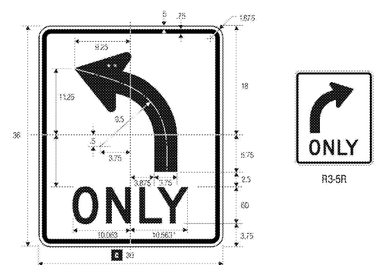
R3-5R RIGHT TURN ONLY SIGN NOT TO SCALE
