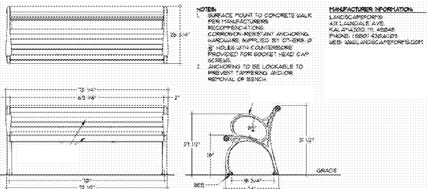
BENCH DETAIL NOT TO SCALE
