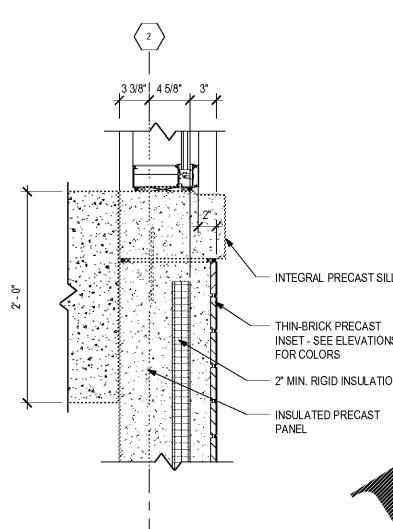
5 SECTION DETAIL A-6.52 1 1/2" = 1'-0"
