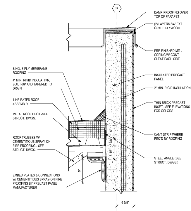
2 SECTION DETAIL A-6.52 1 1/2" = 1'-0"
