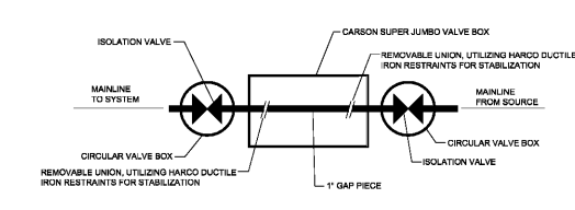
A AIR GAP ASSEMBLY NTS
