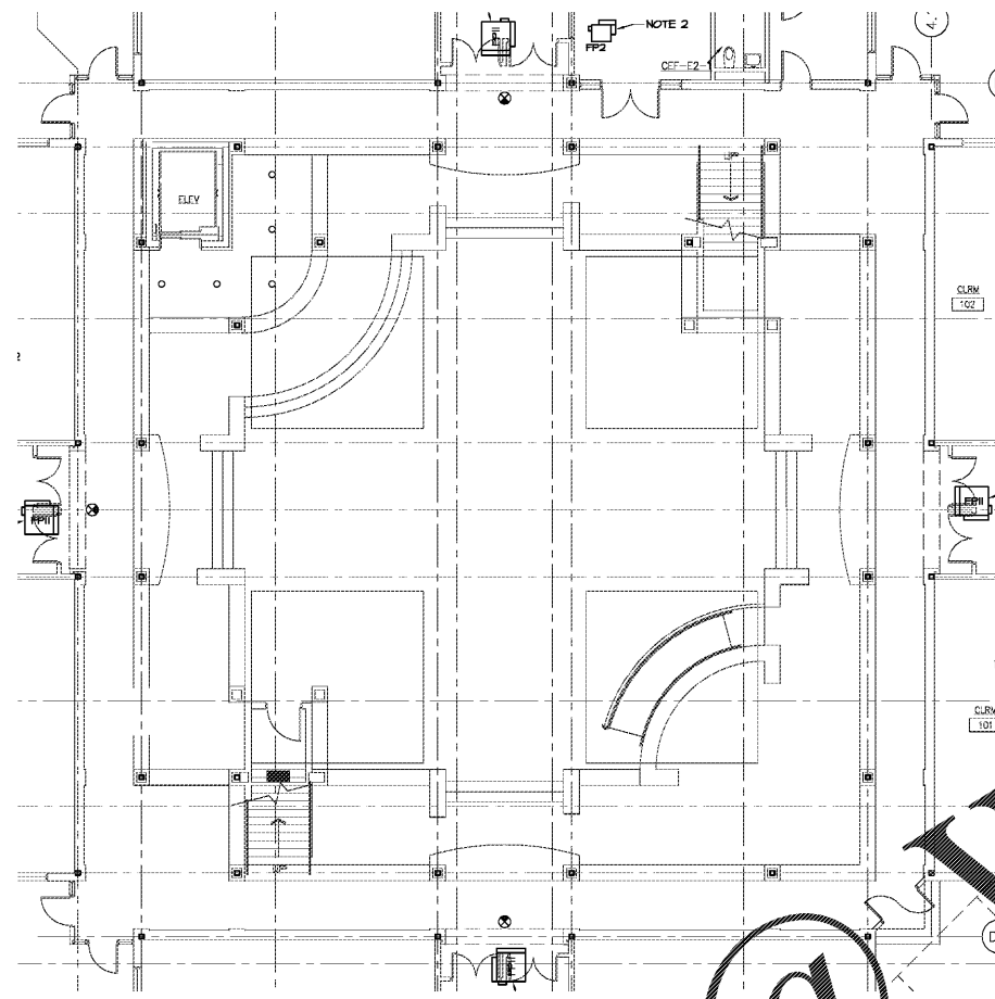
1 PARTIAL FLOOR PLAN - BLDG E - FIRST FLOOR - COMMONS - ELECTRICAL E1.13 1/8"=1'-0"
