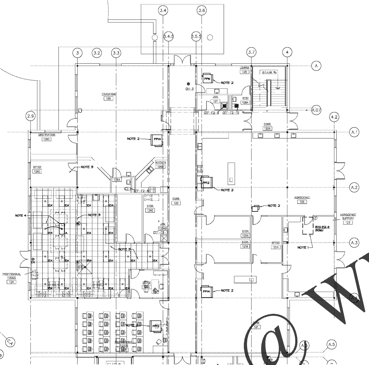
1 PARTIAL FLOOR PLAN - BLDG E - FIRST FLOOR - WING 2 - ELECTRICAL E1.9 1/8"=1'-0"
