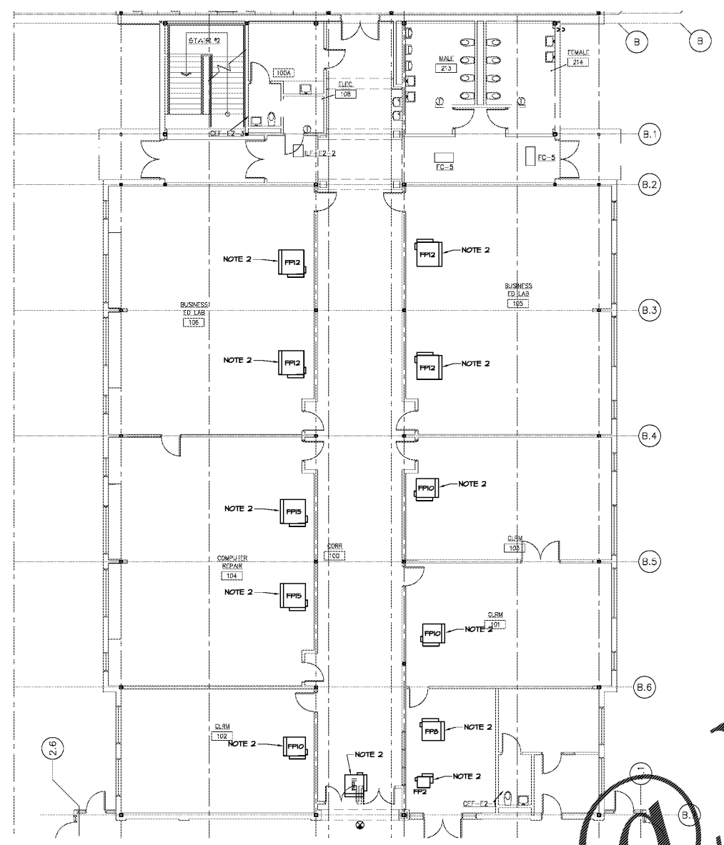
1 PARTIAL FLOOR PLAN - BLDG E - FIRST FLOOR - WING 2 - ELECTRICAL E1.8 1/8"=1'-0"
