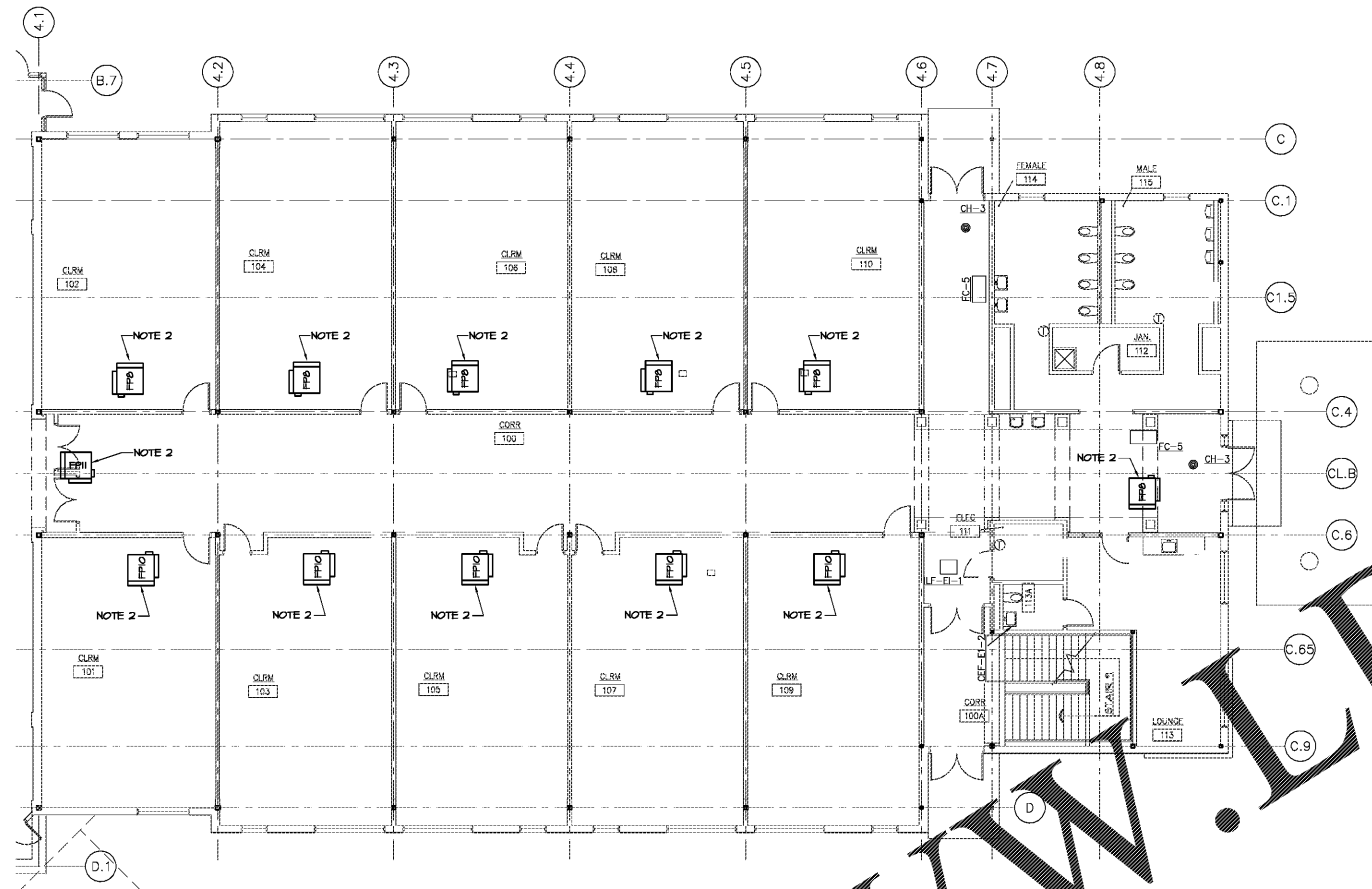
1 PARTIAL FLOOR PLAN - BLDG E - FIRST FLOOR - WING I - ELECTRICAL E1.7 1/8"=1'-0"
