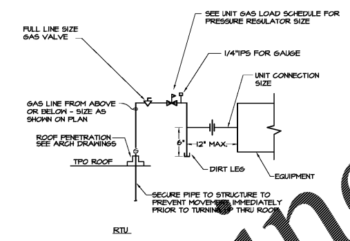
1 TYPICAL GAS CONNECTION DETAIL P2.1 NO SCALE SCHEMATIC ONLY
