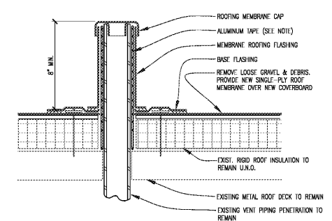
C7 DETAIL WASTE VENT TO REMAIN A-4.10 3'-1'-0"
