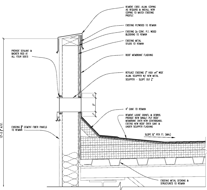
E4 ROOF SCUPPER DETAIL A-4.10 3'-1'-0"
