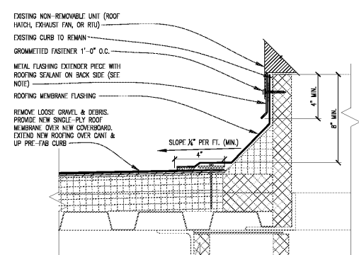
C1 EXISTING NON-REMOVABLE ROOF UNIT DETAIL A-4.10 3'-1'-0"
