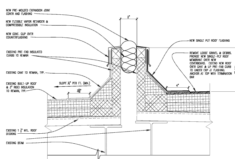
E1 EXPANSION JT. DETAIL A-4.10 3'-1'-0"
