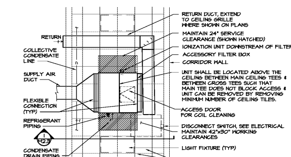
PARTIAL PLAN AT TYPICAL VRF FAN-COIL UNIT
