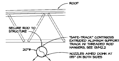
SECTION AT FABRIC DUCT
