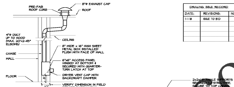
DRYER VENT DETAIL
