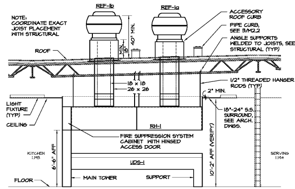
SECTION AT RANGEHOOD
