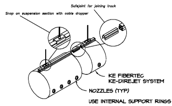
SafeTrack 360° Suspension Detail
