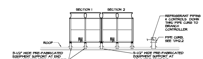
SECTION AT TYPICAL VRF HEAT PUMP ON ROOF
