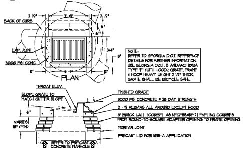
3 G.D.O.T. STANDARD 1019A CURB INLET - TYPE "E" WITH HOOD NOT TO SCALE
