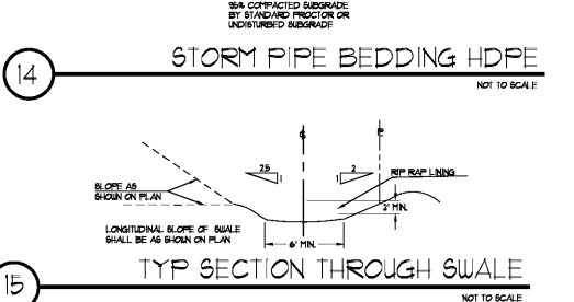
15 TYP SECTION THROUGH SWALE NOT TO SCALE
