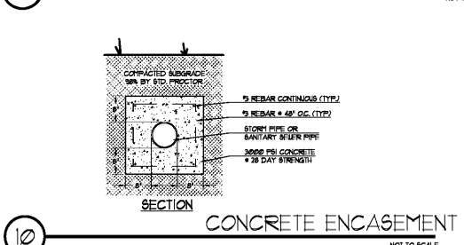
10 CONCRETE ENCASEMENT NOT TO SCALE
