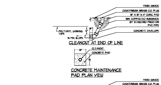
11 CLEANOUT AT END OF LINE NOT TO SCALE
