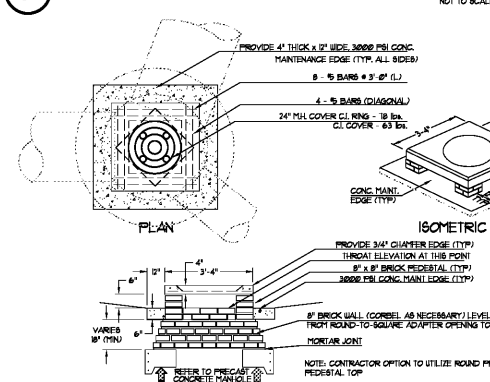
4 PRECAST DROP INLET (D.I.) NOT TO SCALE
