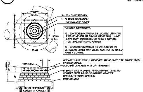
2 JUNCTION BOX / MANHOLE TOP NOT TO SCALE
