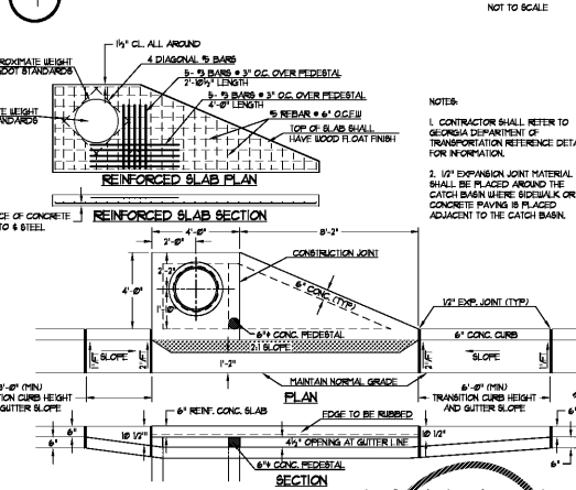
8 G.D.O.T. STANDARD 033 SINGLE-WING CATCH BASIN NOT TO SCALE
