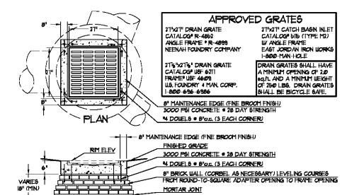
1 21" x 21" CATCH BASIN GRATE & FRAME NOT TO SCALE
