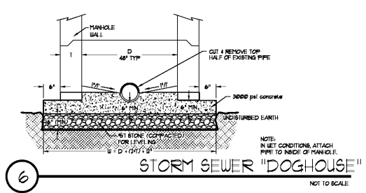
6 STORM SEWER "DOGHOUSE" NOT TO SCALE
