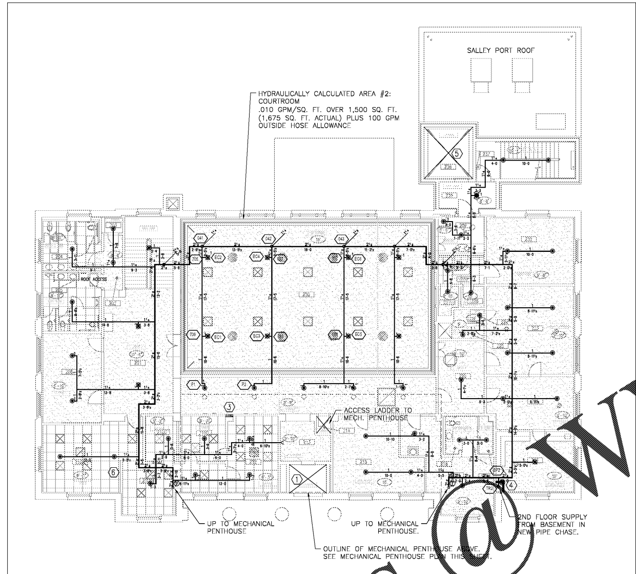
2ND FLOOR FIRE SPRINKLER LAYOUT
