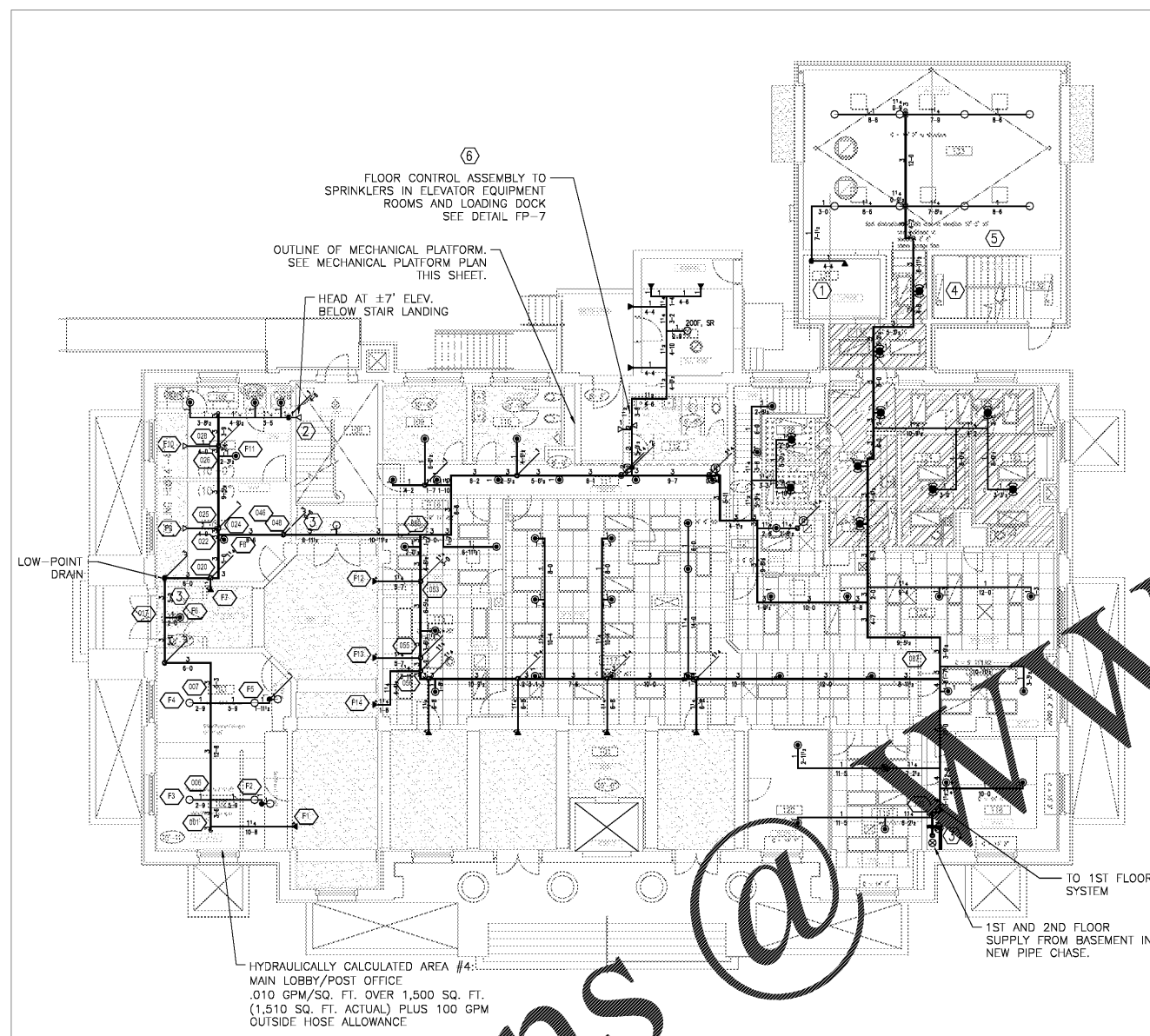
1ST FLOOR FIRE SPRINKLER LAYOUT
