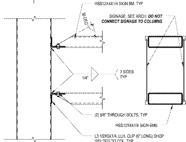
1 SIGNAGE SUPPORT CS4 1'-0\"/>
