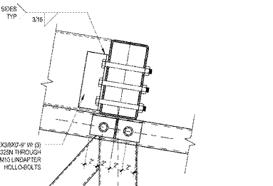
2 COLUMN TO TRUSS CONNECTION CS4 1'-0\"/>
