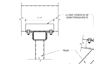
9 HIGH REAR OUTRIGGER TO TRUSS CONNECTION CS4 1'-0\"/>
