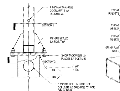
2 COLUMN TO TRUSS CONNECTION CS4 1'-0\"/>
