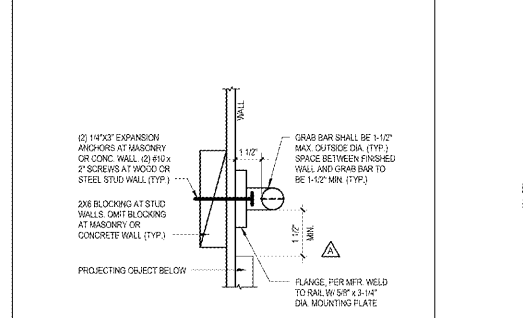
27 GRAB BAR DETAIL ACI 12\"/>
