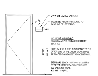
18 TACTILE EXIT SIGNAGE MOUNTING ACI 12\"/>
