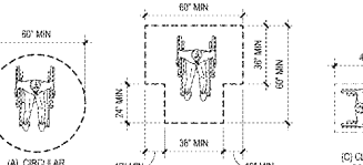
9 CLEAR TURNING SPACE ACI 12\"/>
