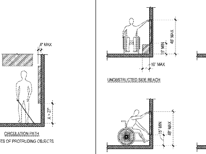
26 PROTRUDING OBJECTS ACI 12\"/>
