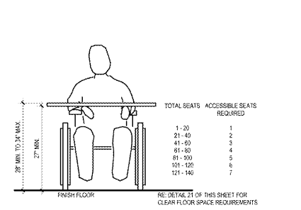
20 SEATING CLEARANCE - FRONT ACI 12\"/>
