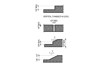
5 CHANGES IN LEVEL ACI 11\"/>
