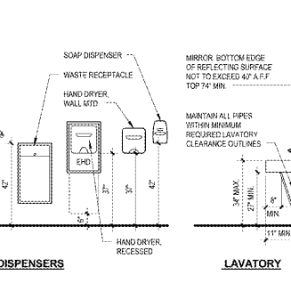
28 DISPENSERS ACI 12\"/>
