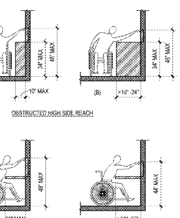
25 ACCESSIBLE REACH ACI 12\"/>
