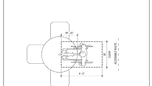
21 SEATING CLEARANCES ACI 12\"/>
