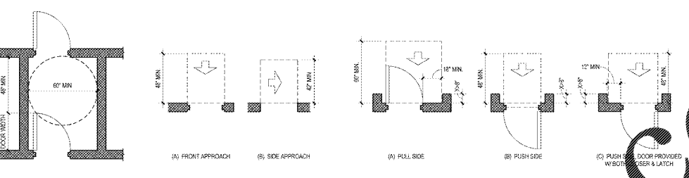
8 MANEUVERING CLEARANCE AT DOORS AND DOORWAYS ACI 12\"/>
