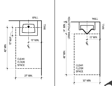
24 ACCESSIBLE LAV. PLAN ACI 12\"/>
