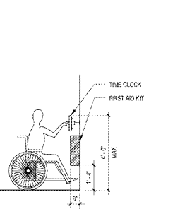
19 TIME CLOCK ACCESSIBLE REACH ACI 12\"/>
