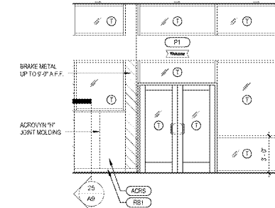
2 FRONT VESTIBULE ELEVATION A8.2 10' x 10'
