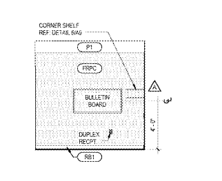
10 OFFICE ELEVATION A8.2 10' x 10'
