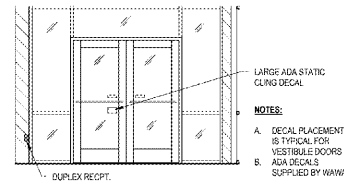
5 ADA DECAL DTL @ VESTIBULE DOOR A8.2 10' x 10'
