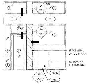
4 FRONT VESTIBULE ELEVATION A8.2 10' x 10'
