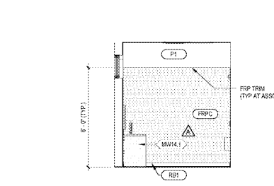
16 ASSOCIATE'S ROOM ELEV. A8.2 10' x 10'
