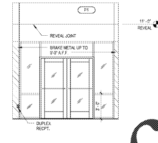
1 FRONT VESTIBULE ELEVATION A8.2 10' x 10'
