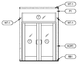
8 REAR VESTIBULE ELEVATION A8.2 10' x 10'
