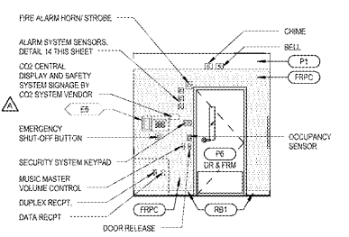
11 OFFICE ELEVATION A8.2 10' x 10'
