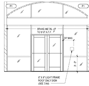
3 FRONT VESTIBULE ELEVATION A8.2 10' x 10'
