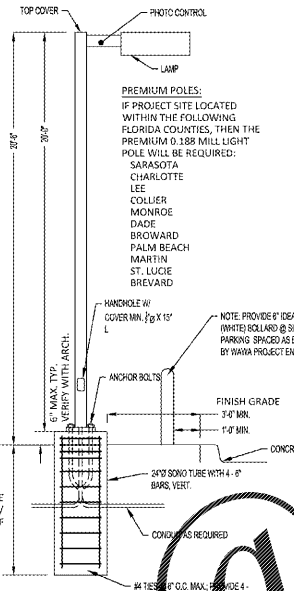
LIGHT POLE WITH STANDARD ANCHOR AND SEAL NTS
