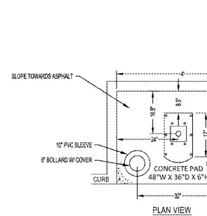
AIR PUMP STAND NTS
