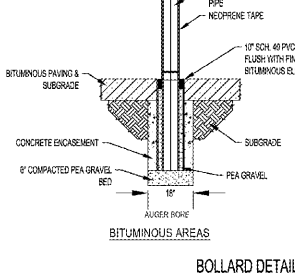
BITUMINOUS AREAS NTS
