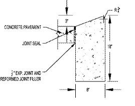
WAWA TYPE B1 CURB NTS
