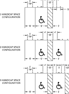
BOLLARD SPACING/DIMENSION DETAIL NTS
