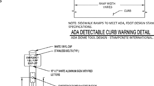
EMERGENCY PUMP SHUTOFF DETAIL NTS
