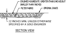
SECTION VIEW NTS
