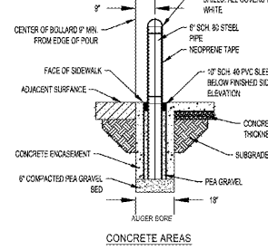
CONCRETE AREAS NTS
