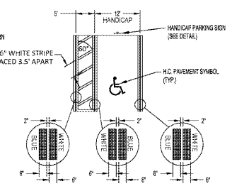
HANDICAP STRIPING DETAIL NTS
