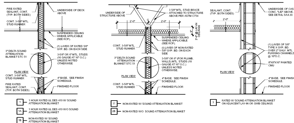
2 PARTITION TYPES SCALE: 3/4" = 1'-0"
