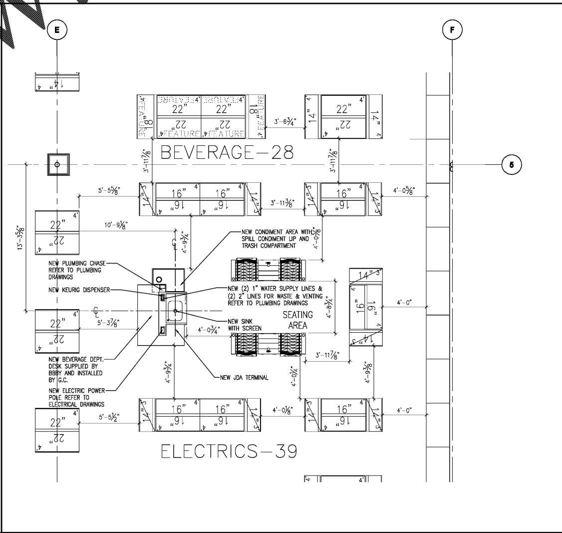
ENLARGED FIXT. PLAN - BEV. / ELECTRICS / COOKWARE 01
