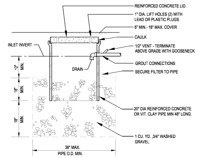
3 TYPICAL DRYWELL DETAIL NOT TO SCALE
