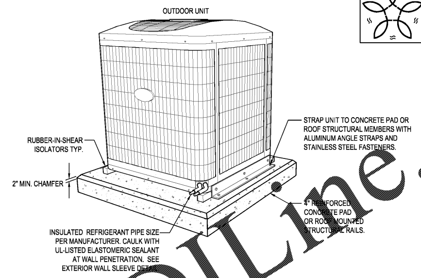
1 TYPICAL OUTDOOR UNIT MOUNTING DETAIL NOT TO SCALE
