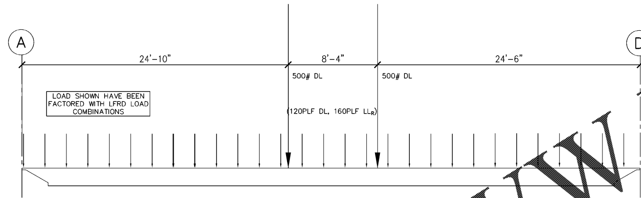
2 SPECIAL JOIST 2 LOADING DIAGRAM S3.2 SCALE: 1/4" = 1'-0"
