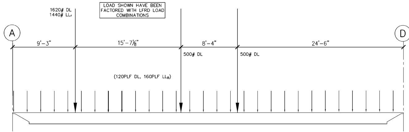
1 SPECIAL JOIST 1 LOADING DIAGRAM S3.2 SCALE: 1/4" = 1'-0"
