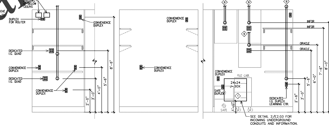
3 POS ELEVATIONS AT OFFICE E2.03 SCALE: 1/2"=1'-0"
