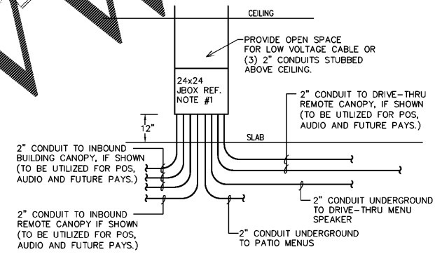
2 POS JBOX DIAGRAM E2.03 SCALE: NONE
