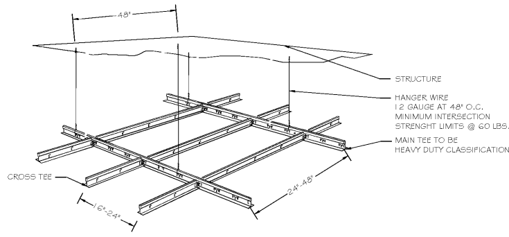
1 ISOMETRIC DETAIL NOT TO SCALE
