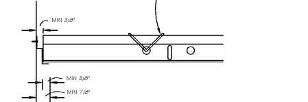
Figure 3. Seismic detail of suspended ceiling showing the hanger wire perimeter supports two alternatives:
