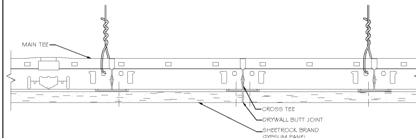
8 GYPSUM SOFFIT AT SUSPENDED CEILING, TYP. NOT TO SCALE
