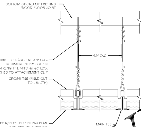
4 ATTACHMENT DETAIL NOT TO SCALE
