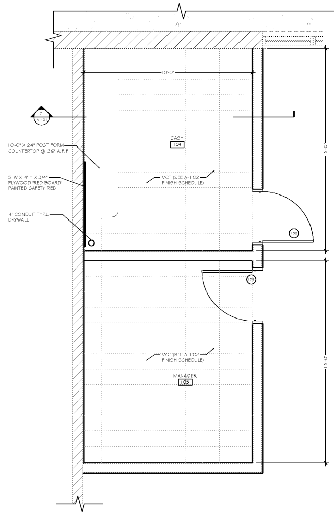
1 ENLARGED PLAN @ CASH/MANAGER 3/8" = 1'-0"
