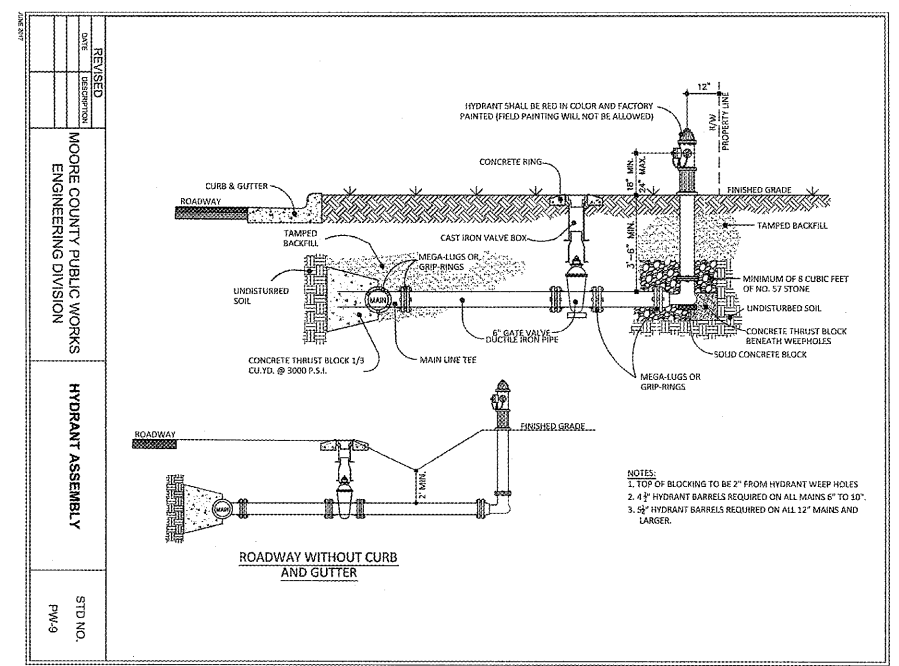
FIRE HYDRANT DETAIL N.T.S. 1 US3
