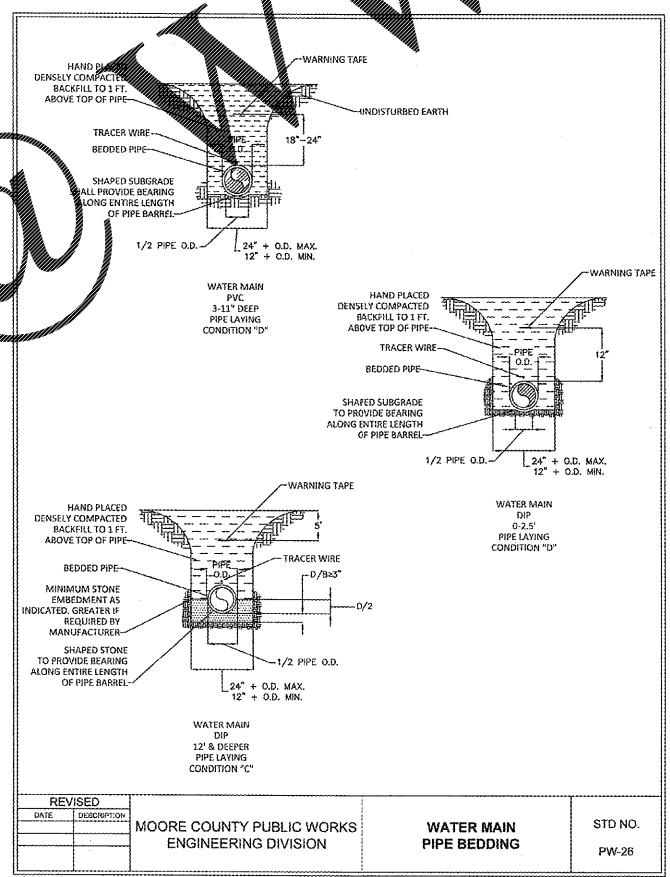
WATER MAIN PIPE BEDDING DETAIL N.T.S. 2 US3
