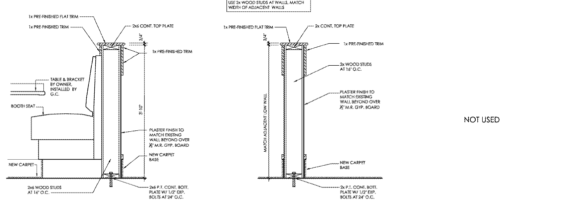
14, 15, 16 LOW WALL DETAIL 1"
