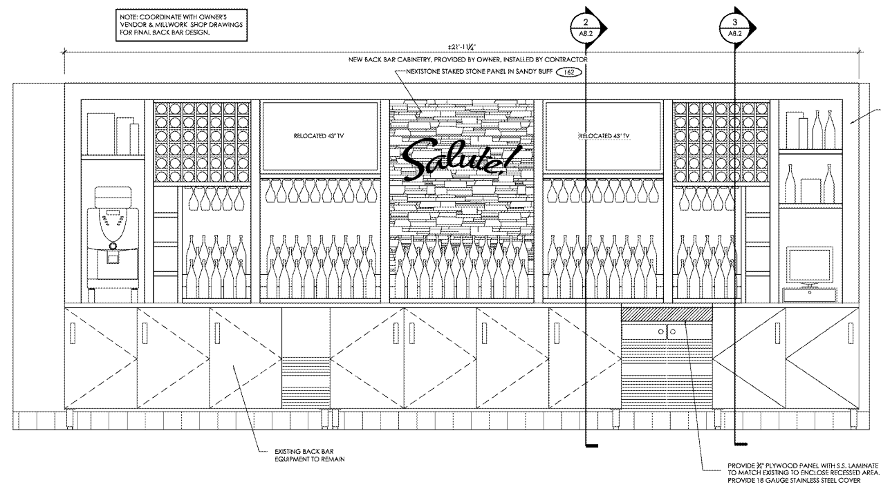
1 BACK BAR ELEVATION 3/4"
