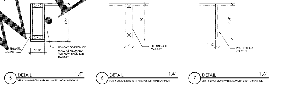
4 DETAIL 1 1/2" 5 DETAIL 1 1/2" 6 DETAIL 1 1/2" 7 DETAIL 1 1/2"
