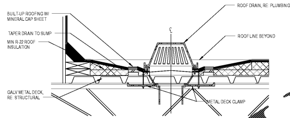
7 Roof Drain & Overflow Assembly 2 SCALE: 1 1/2" = 1'-0"
