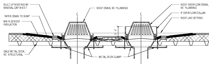
6 Roof Drain & Overflow Assembly 1 SCALE: 1 1/2" = 1'-0"
