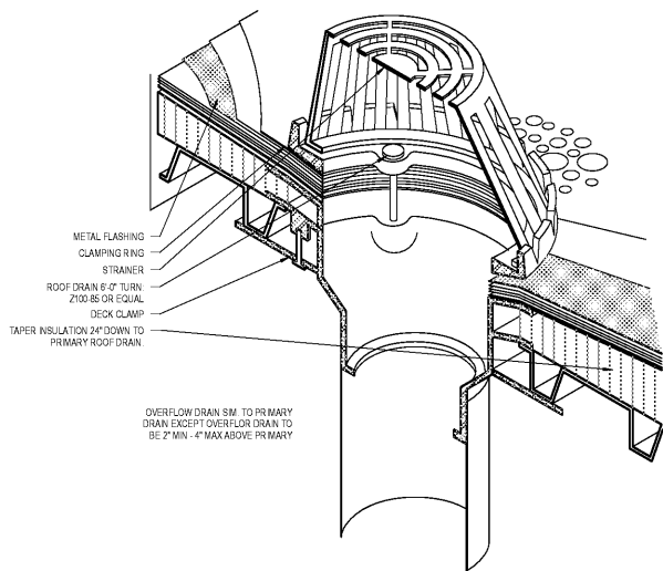
1 Roof Drain Detail SCALE: 1 1/2" = 1'-0"
