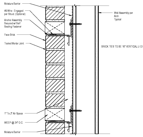
14 Veneer w/ Steel Stud @ Wall SCALE: 3" = 1'-0"
