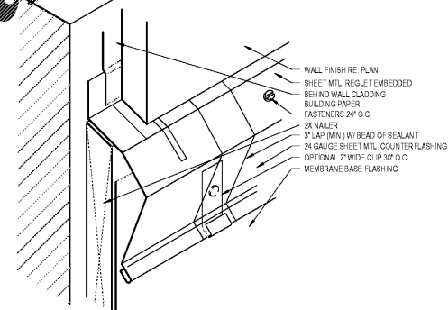
12 Flashing Detail SCALE: 3/4" = 1'-0"
