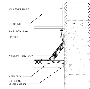
15 Parapet Roof Flashing Detail SCALE: 1 1/2" = 1'-0"
