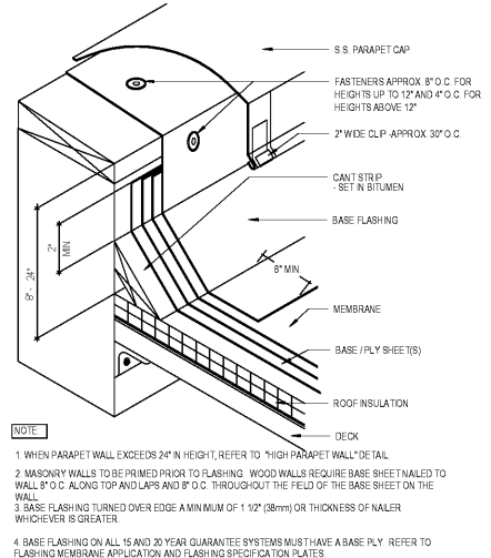
3 Low Wall Flashing Detail SCALE: 1 1/2" = 1'-0"
