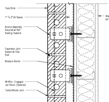
13 Brick Veneer on Stud (Plan) SCALE: 3" = 1'-0"
