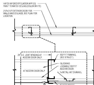
10 Access Hatch & Lock Detail SCALE: 1 1/2" = 1'-0"
