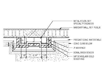
22 Pilaster at 4'-0" SCALE: 1/2" = 1'-0"
