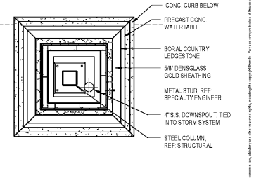
24 Column at 6'-0" SCALE: 1/2" = 1'-0"
