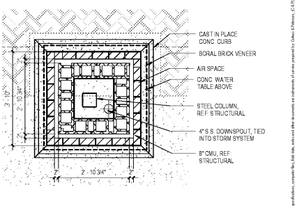
23 Column at 2'-0" SCALE: 1/2" = 1'-0"
