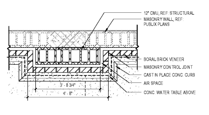
21 Pilaster at 2'-0" SCALE: 1/2" = 1'-0"
