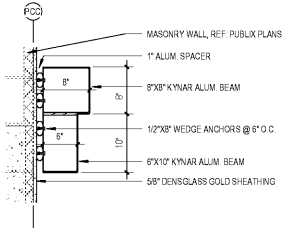
20 Kynar Double Beam Profile SCALE: 1" = 1'-0"
